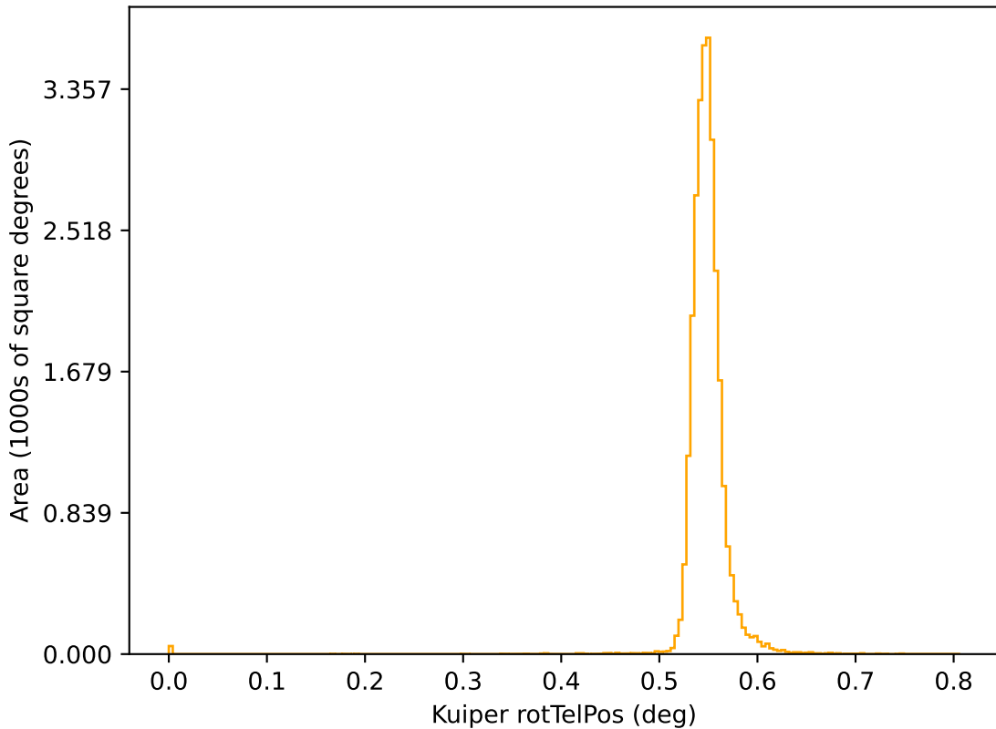
too_elab_r256_d2_griz_v3.4_10yrs r: Kuiper rotTelPos
