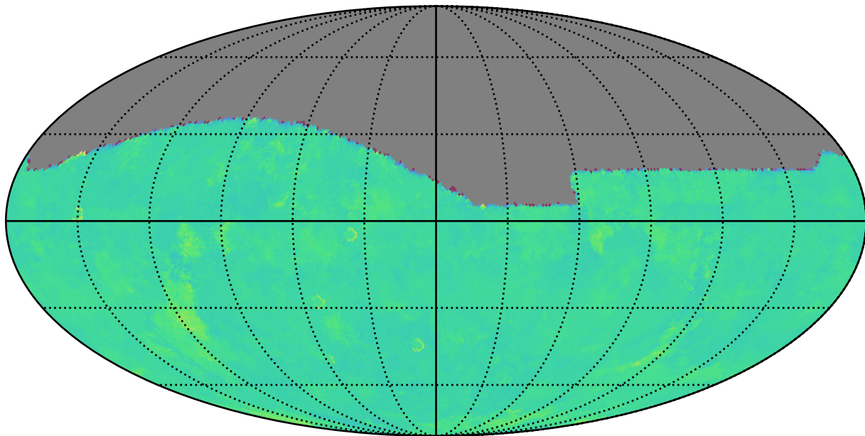
too_elab_r256_d2_griz_v3.4_10yrs g: Kuiper rotTelPos
