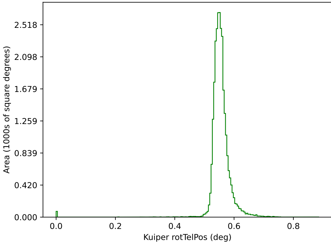
too_elab_r256_d2_griz_v3.4_10yrs g: Kuiper rotTelPos
