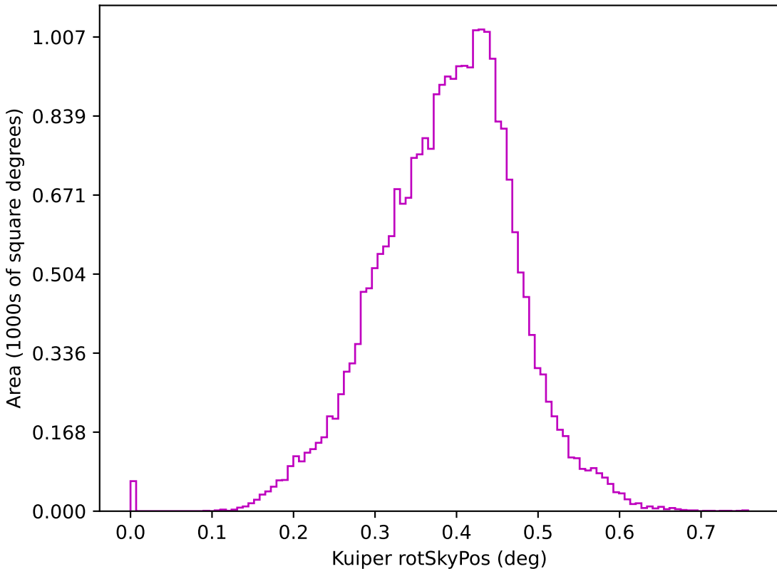
too_elab_r256_d2_griz_v3.4_10yrs z: Kuiper rotSkyPos
