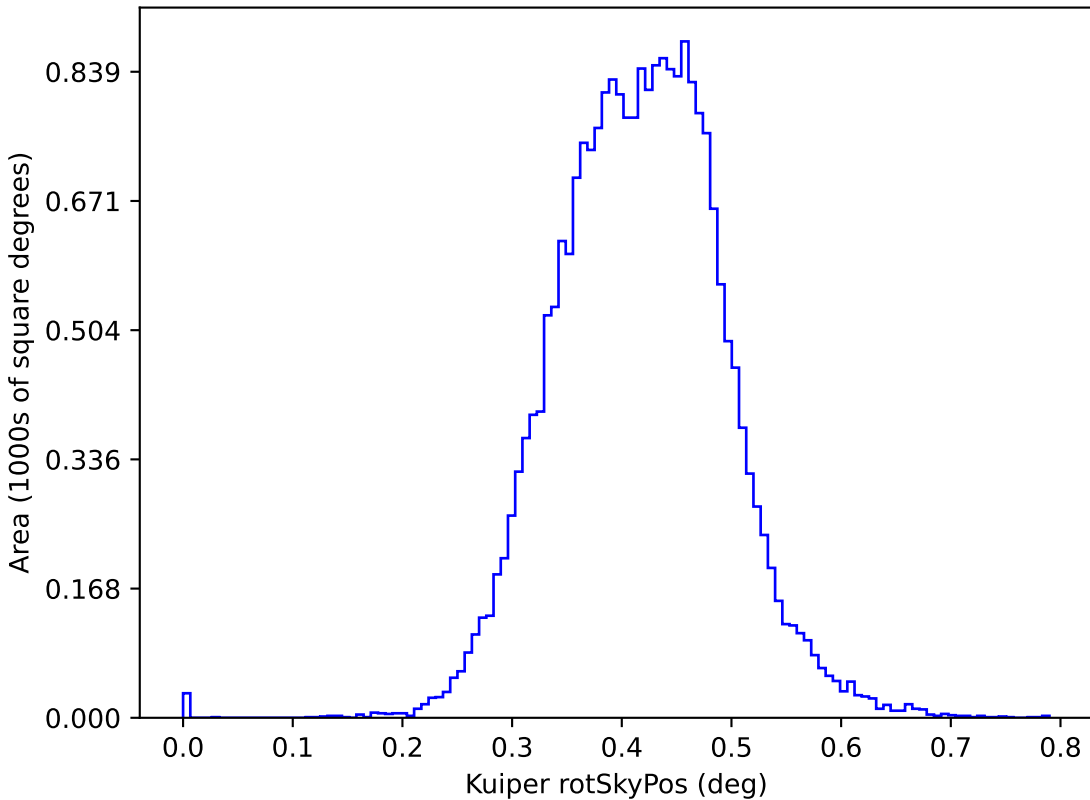
too_elab_r256_d2_griz_v3.4_10yrs y: Kuiper rotSkyPos
