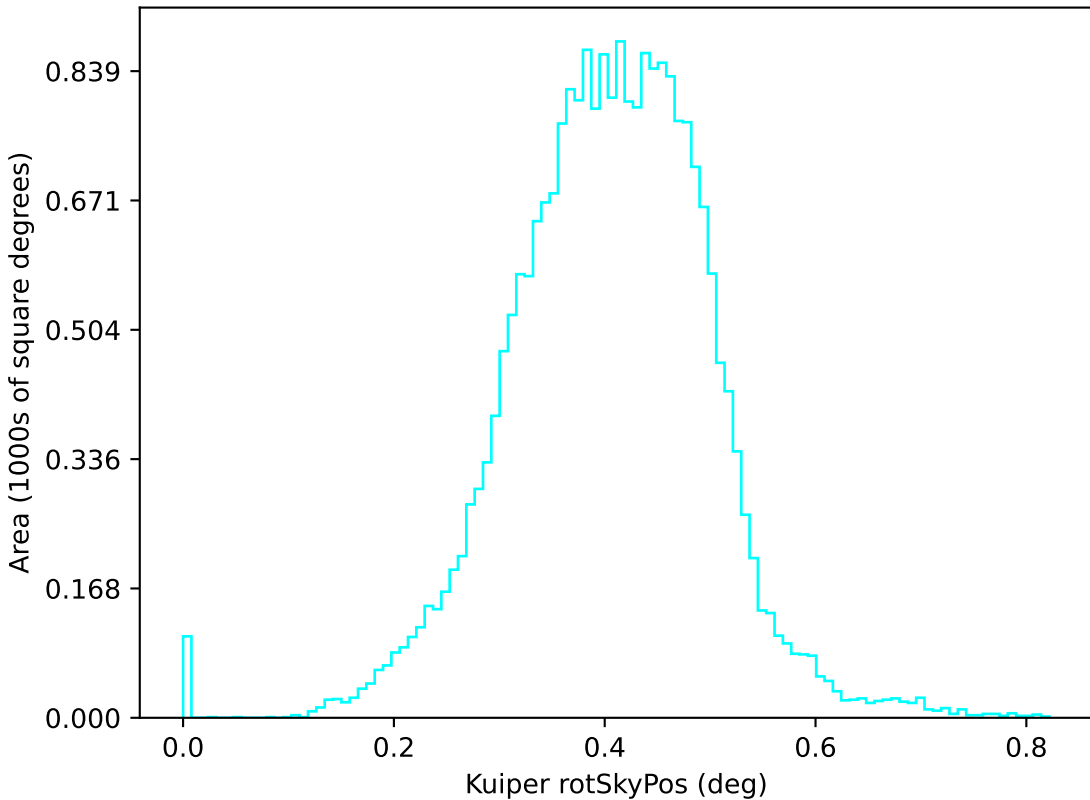
too_elab_r256_d2_griz_v3.4_10yrs u: Kuiper rotSkyPos
