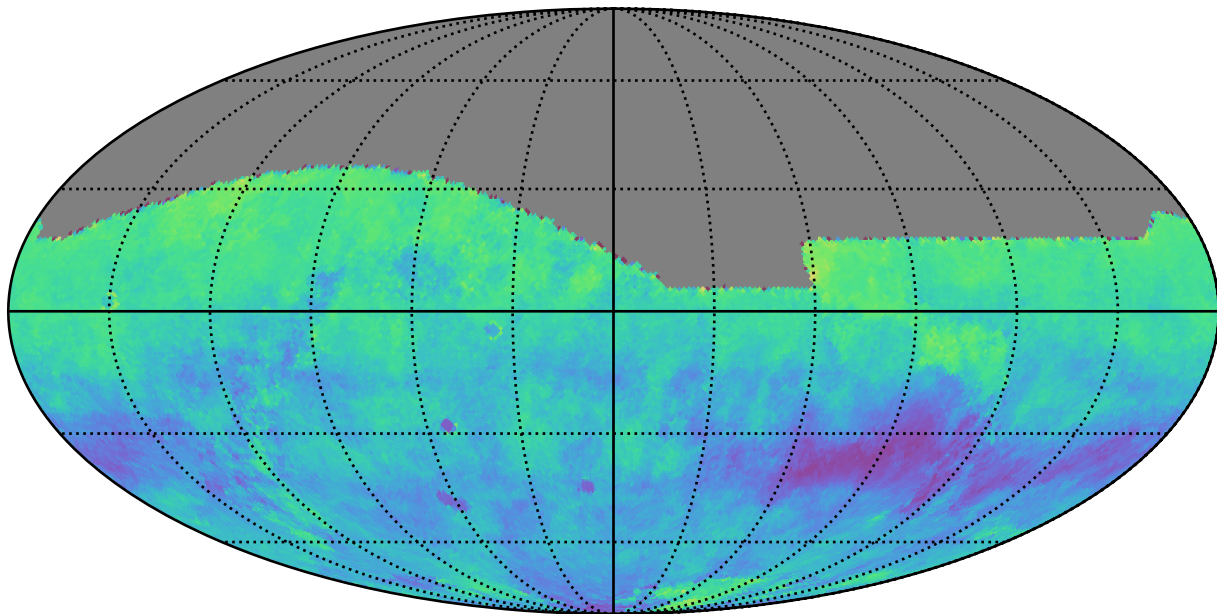
too_elab_r256_d2_griz_v3.4_10yrs r: Kuiper rotSkyPos
