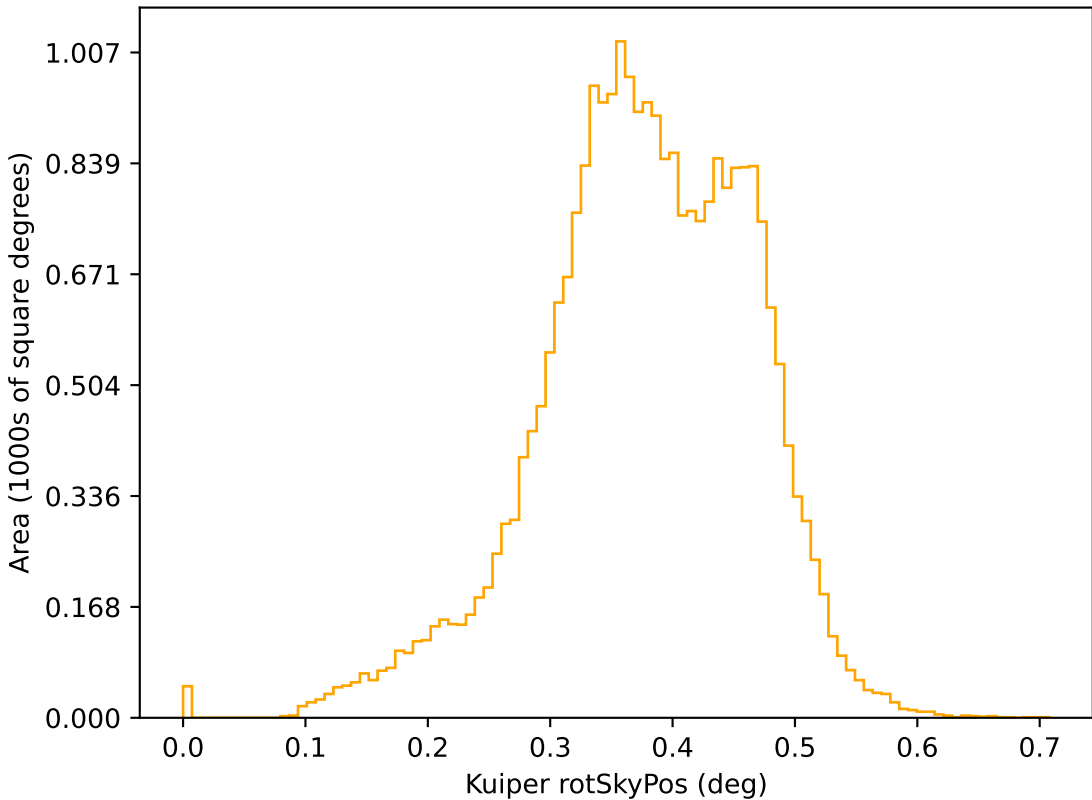
too_elab_r256_d2_griz_v3.4_10yrs r: Kuiper rotSkyPos
