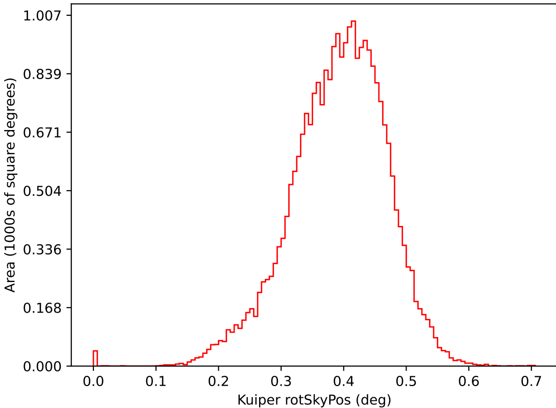
too_elab_r256_d2_griz_v3.4_10yrs i: Kuiper rotSkyPos
