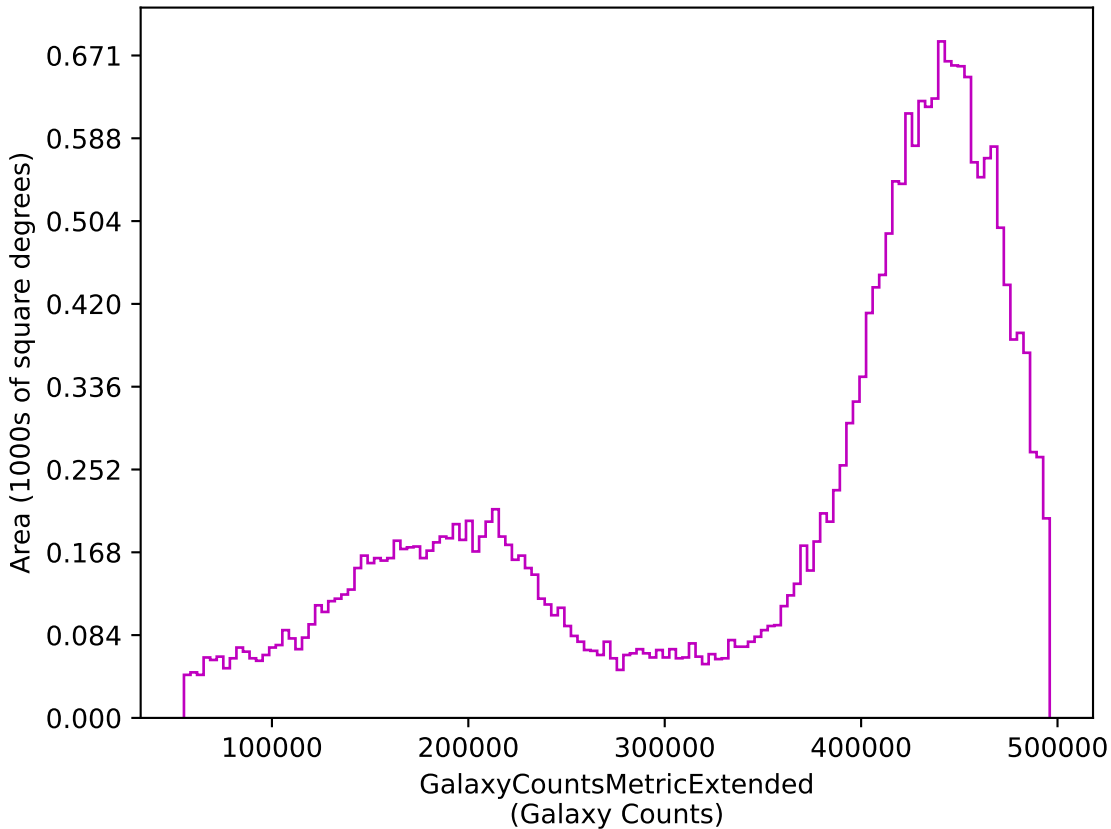
too_elab_r256_d2_griz_v3.4_10yrs z: GalaxyCountsMetricExtended
