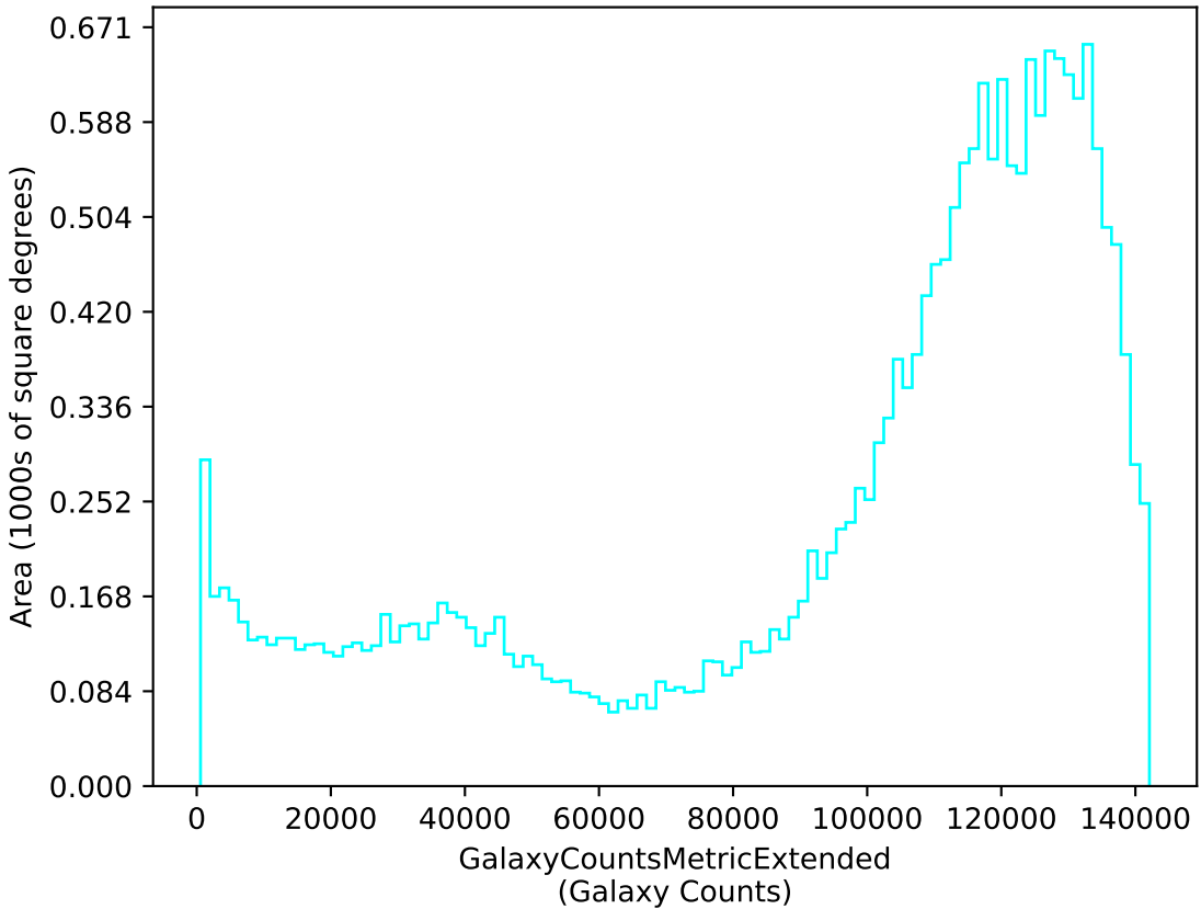
too_elab_r256_d2_griz_v3.4_10yrs u: GalaxyCountsMetricExtended
