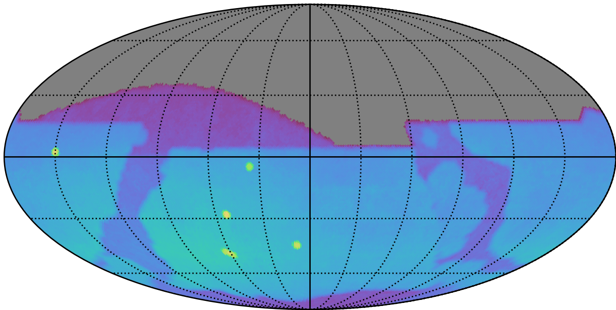
too_elab_r256_d2_griz_v3.4_10yrs : Brown Dwarf, L4
