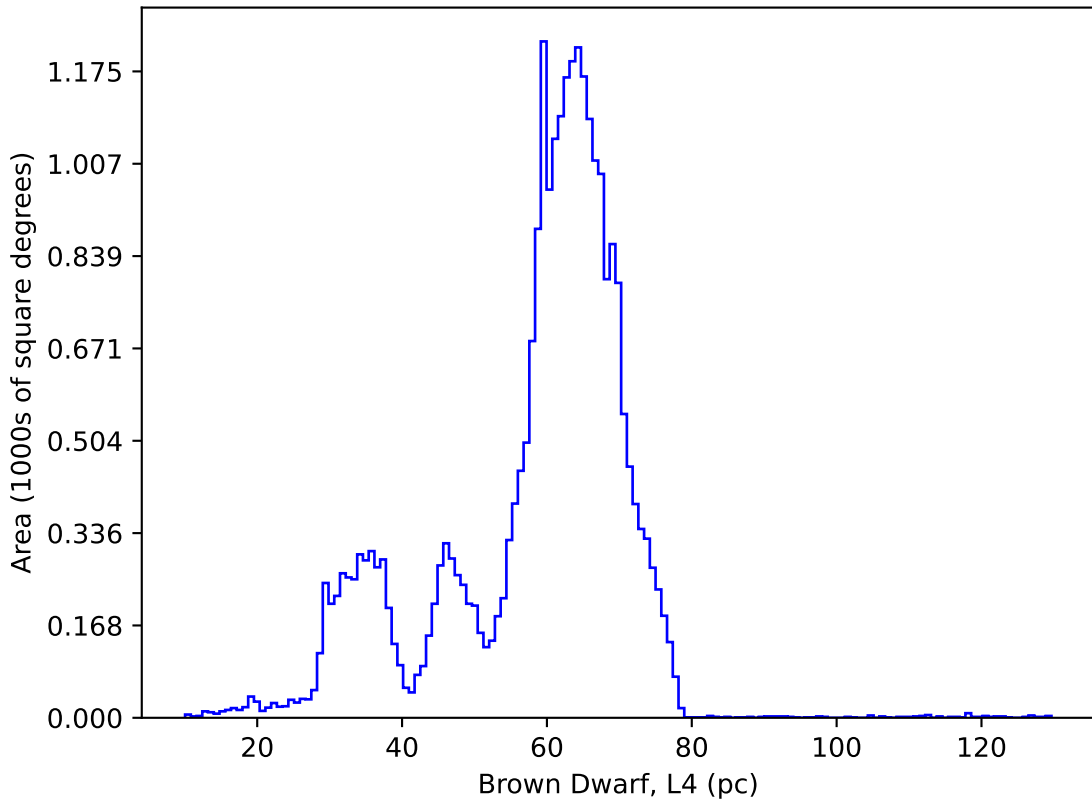
too_elab_r256_d2_griz_v3.4_10yrs : Brown Dwarf, L4
