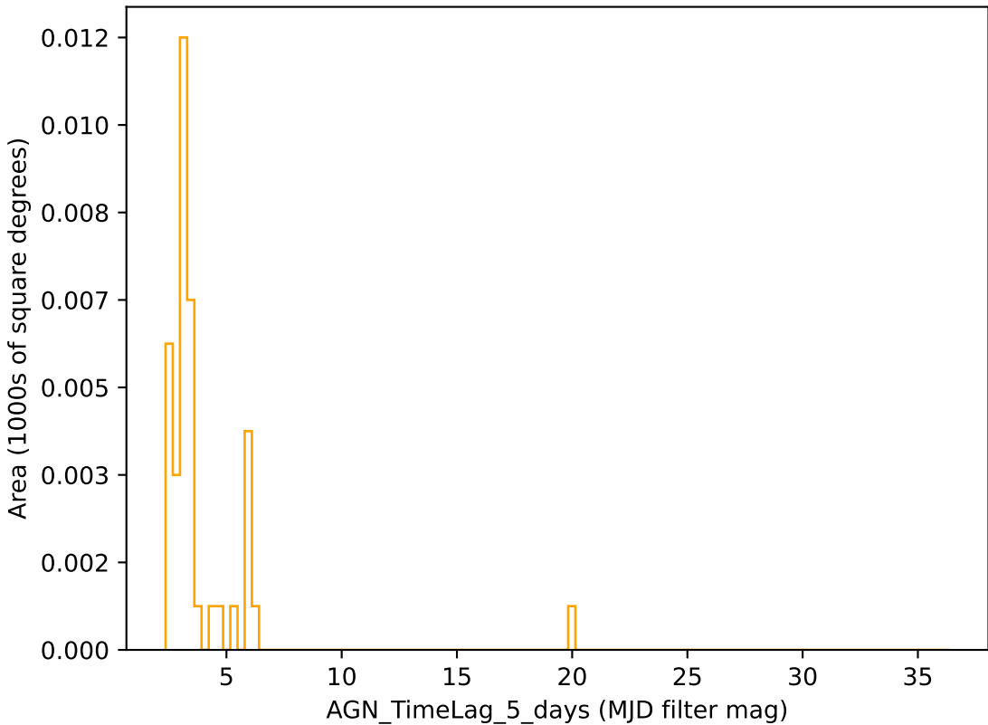
too_elab_r256_d2_griz_v3.4_10yrs r band: AGN_TimeLag_5_days
