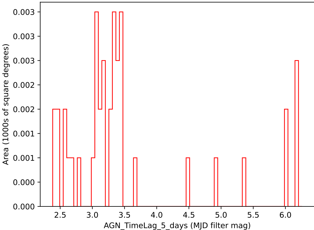
too_elab_r256_d2_griz_v3.4_10yrs i band: AGN_TimeLag_5_days
