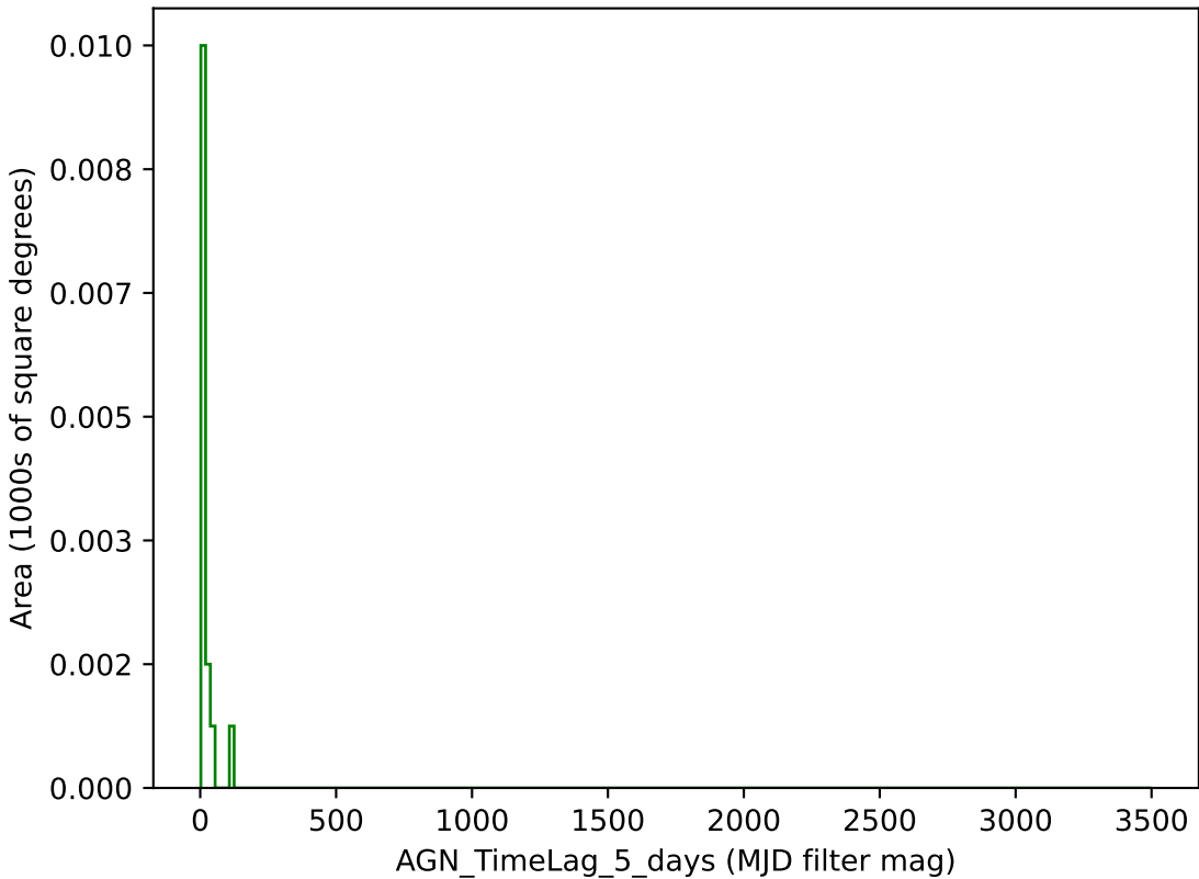
too_elab_r256_d2_griz_v3.4_10yrs g band: AGN_TimeLag_5_days
