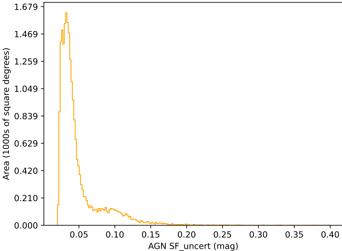
too_elab_r256_d2_griz_v3.4_10yrs r band: AGN SF_uncert
