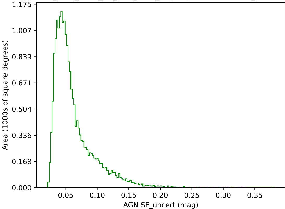
too_elab_r256_d2_griz_v3.4_10yrs g band: AGN SF_uncert
