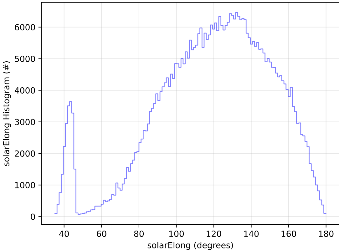
too_elab_r256_d2_griz_v3.4_10yrs WFD z band: solarElong Histogram
