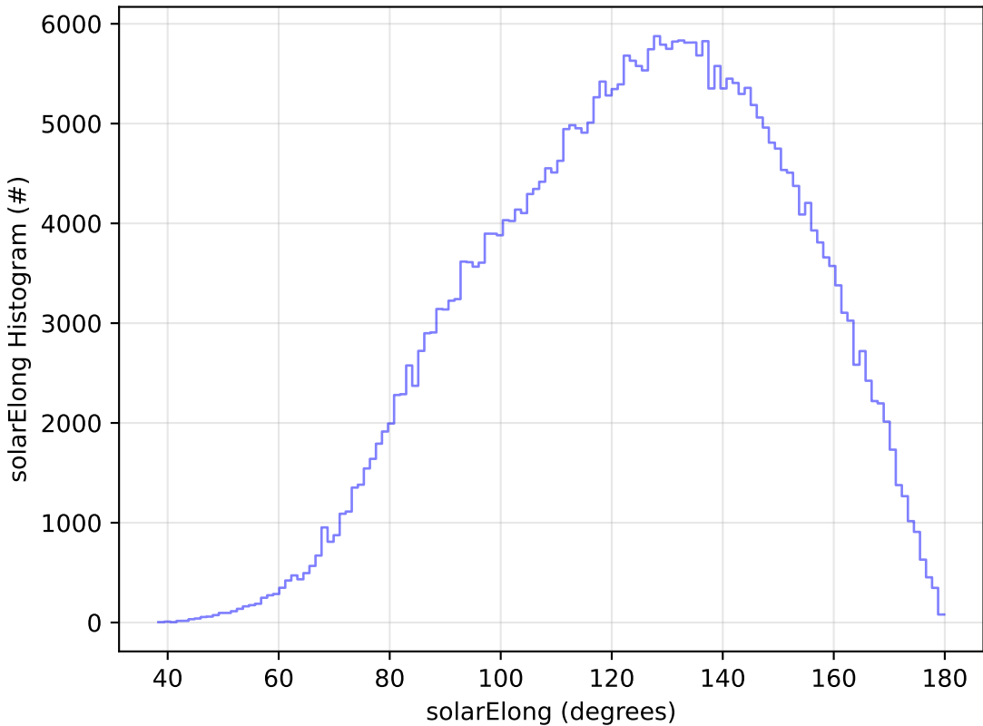
too_elab_r256_d2_griz_v3.4_10yrs WFD y band: solarElong Histogram
