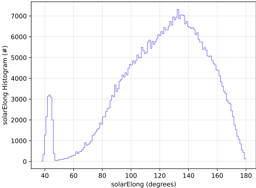
too_elab_r256_d2_griz_v3.4_10yrs WFD r band: solarElong Histogram
