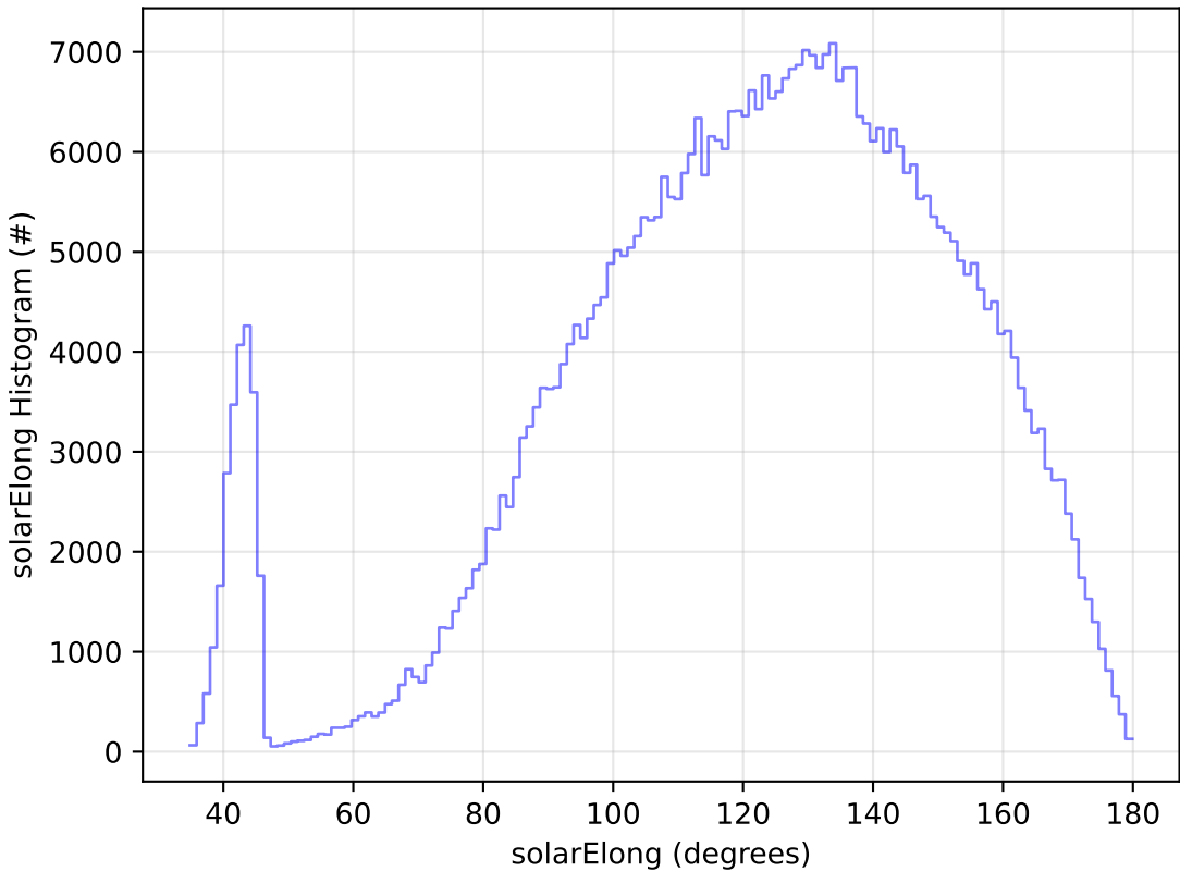
too_elab_r256_d2_griz_v3.4_10yrs WFD i band: solarElong Histogram
