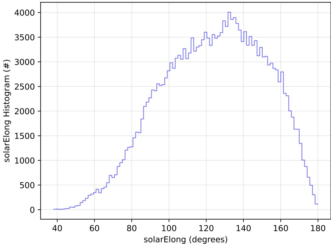
too_elab_r256_d2_griz_v3.4_10yrs WFD g band: solarElong Histogram
