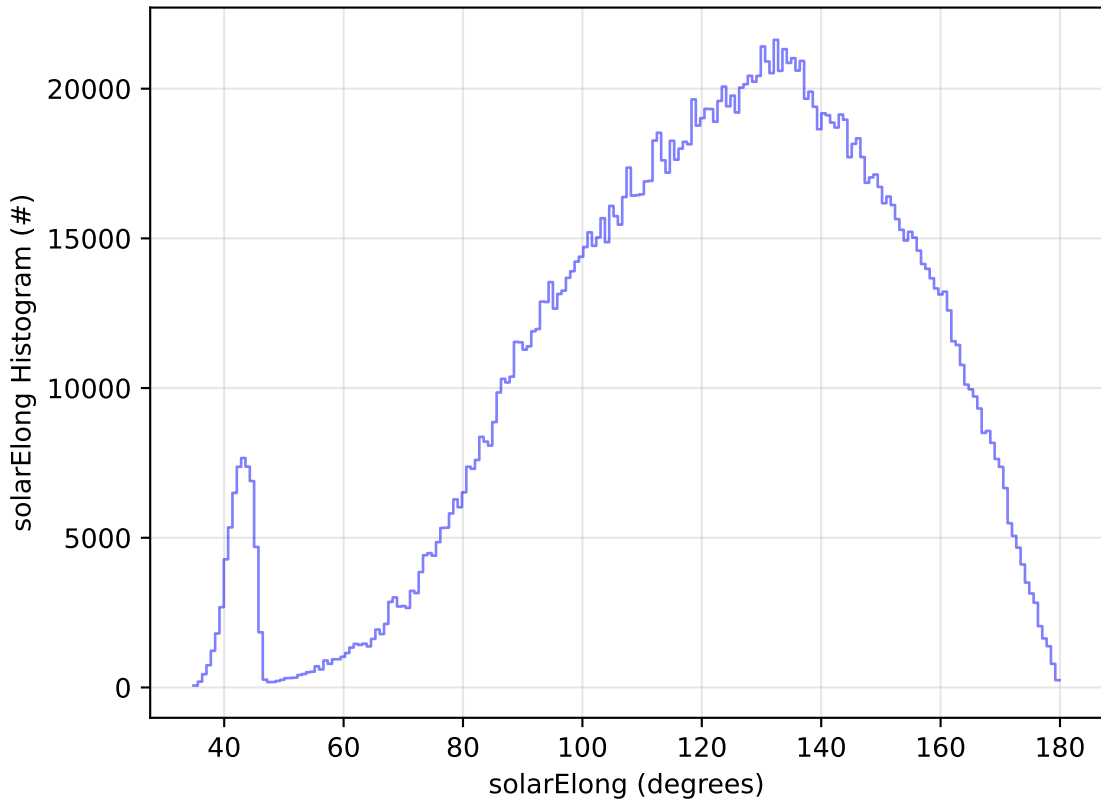
too_elab_r256_d2_griz_v3.4_10yrs WFD all bands: solarElong Histogram
