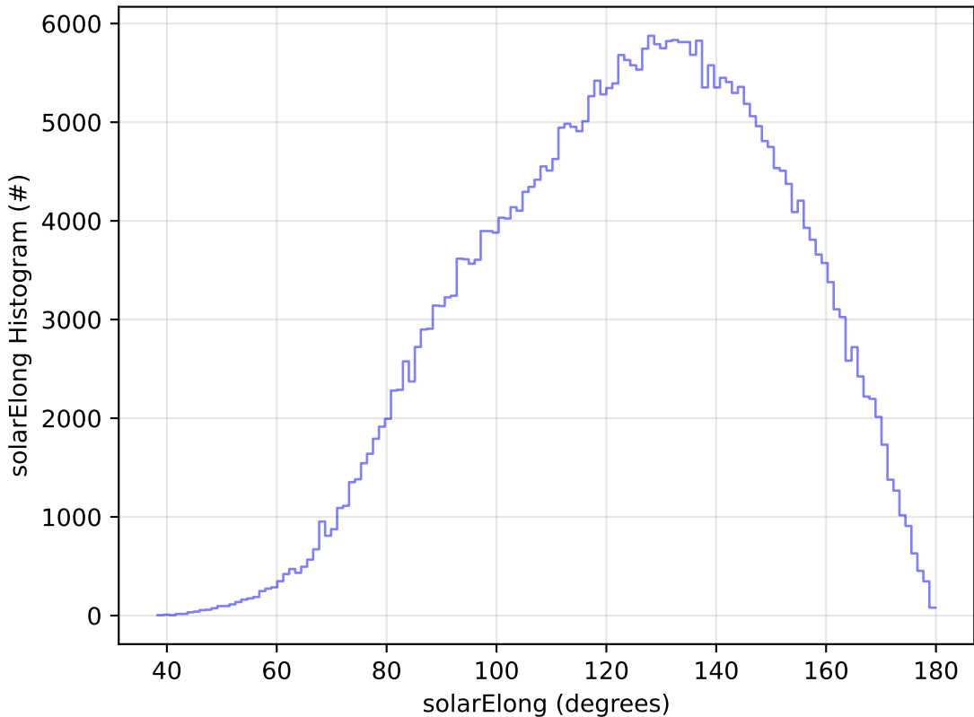
too_elab_r256_d2_griz_v3.4_10yrs All sky y band: solarElong Histogram
