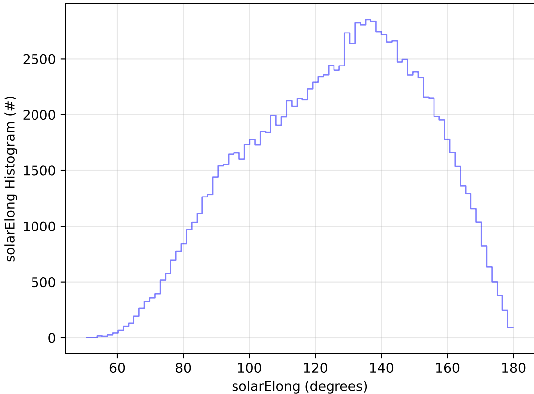
too_elab_r256_d2_griz_v3.4_10yrs All sky u band: solarElong Histogram
