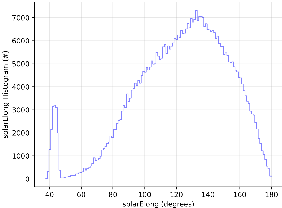
too_elab_r256_d2_griz_v3.4_10yrs All sky r band: solarElong Histogram
