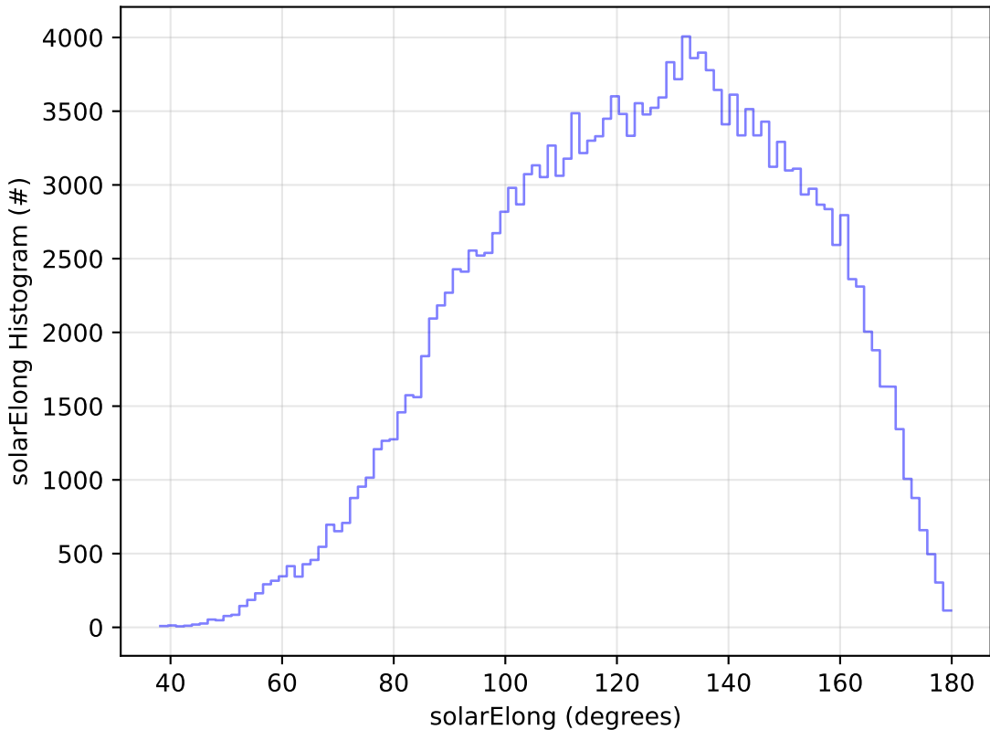
too_elab_r256_d2_griz_v3.4_10yrs All sky g band: solarElong Histogram
