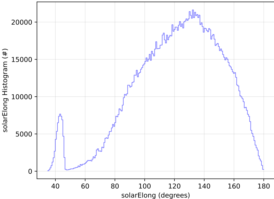
too_elab_r256_d2_griz_v3.4_10yrs All sky all bands: solarElong Histogram
