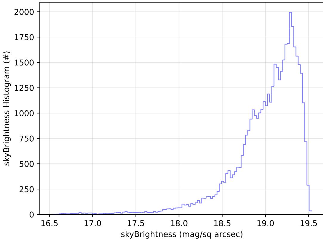
too_elab_r256_d2_griz_v3.4_10yrs Yr 1 z band: skyBrightness Histogram
