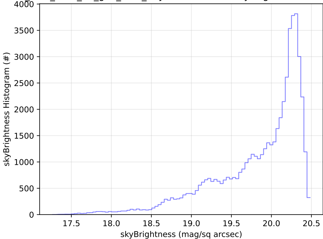
too_elab_r256_d2_griz_v3.4_10yrs Yr 1 i band: skyBrightness Histogram
