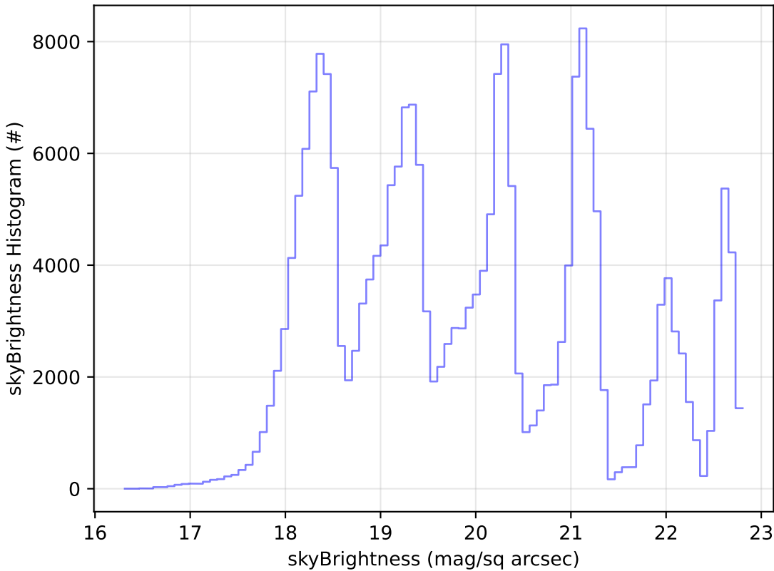
too_elab_r256_d2_griz_v3.4_10yrs Yr 1 all bands: skyBrightness Histogram
