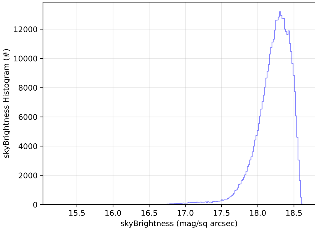
too_elab_r256_d2_griz_v3.4_10yrs WFD y band: skyBrightness Histogram
