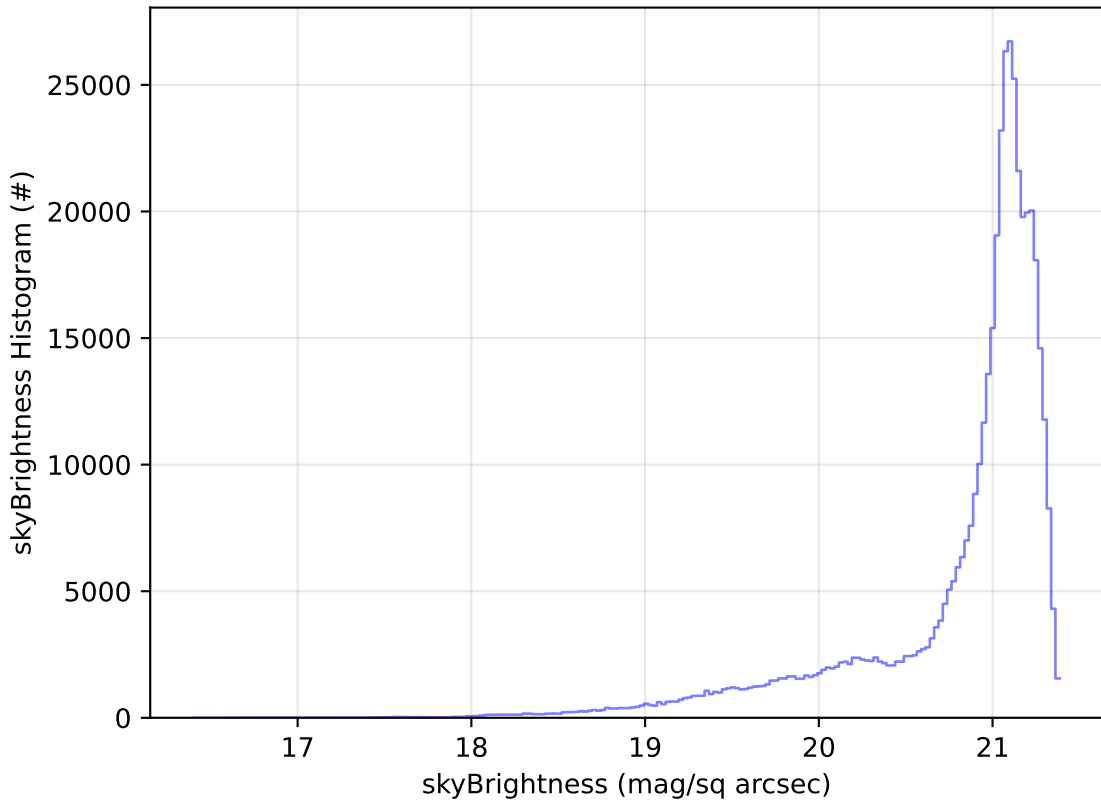
too_elab_r256_d2_griz_v3.4_10yrs WFD r band: skyBrightness Histogram
