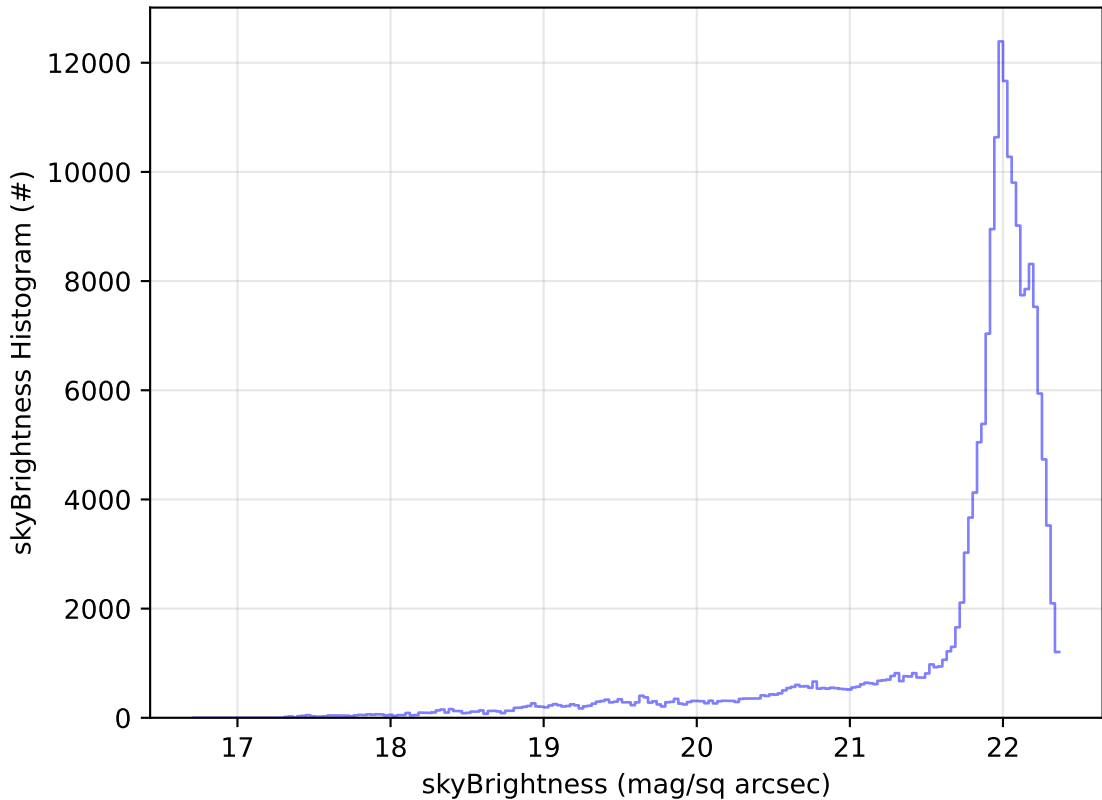
too_elab_r256_d2_griz_v3.4_10yrs WFD g band: skyBrightness Histogram
