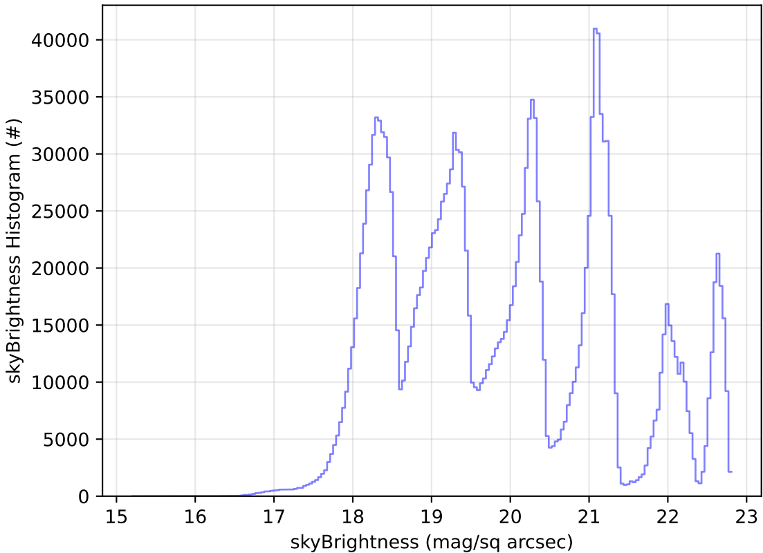
too_elab_r256_d2_griz_v3.4_10yrs WFD all bands: skyBrightness Histogram
