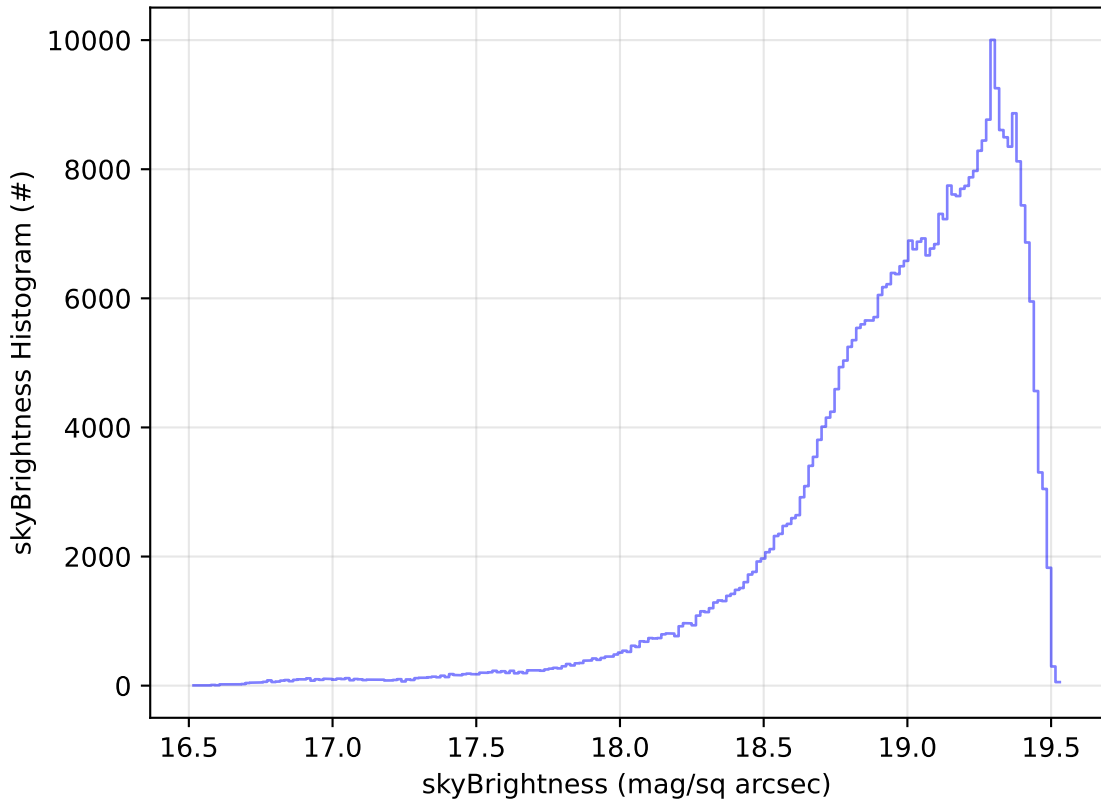
too_elab_r256_d2_griz_v3.4_10yrs All sky z band: skyBrightness Histogram
