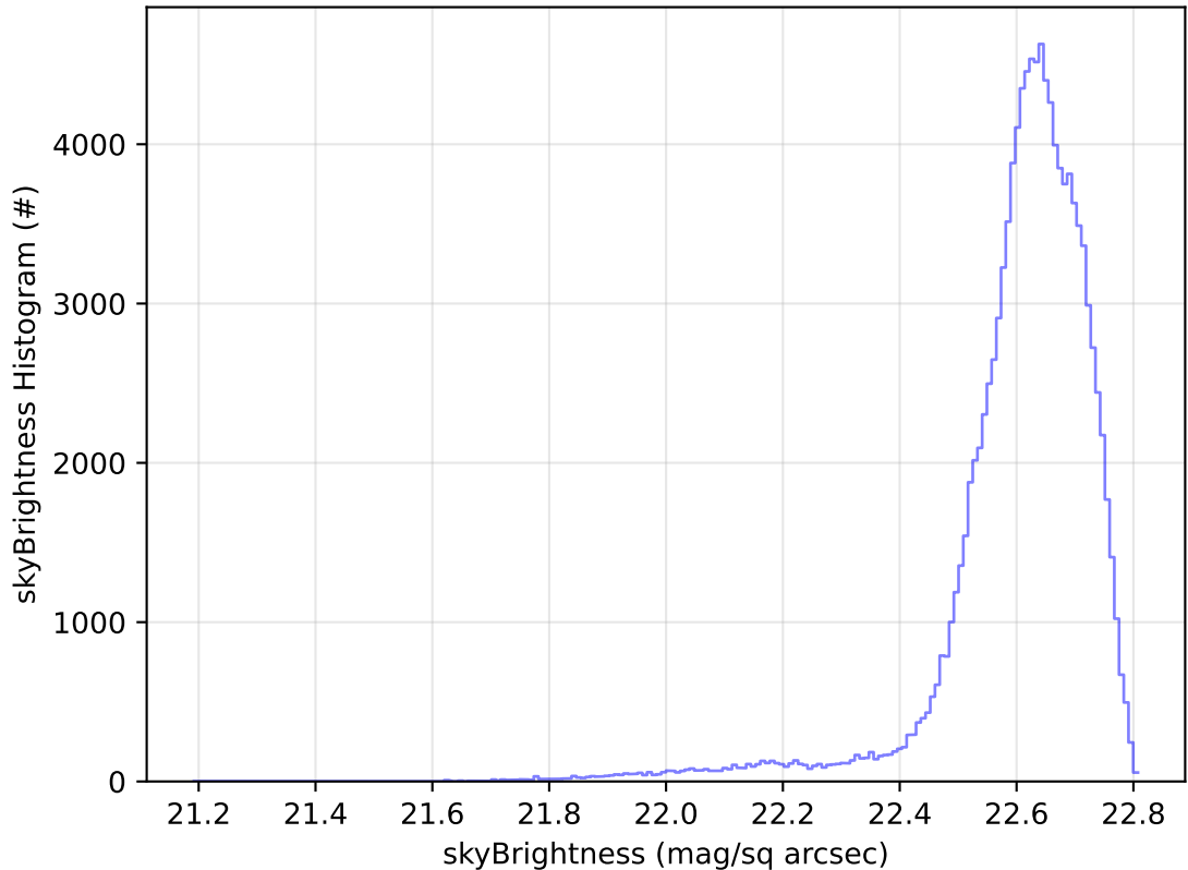
too_elab_r256_d2_griz_v3.4_10yrs All sky u band: skyBrightness Histogram
