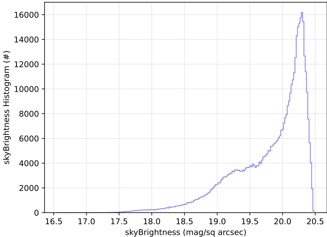
too_elab_r256_d2_griz_v3.4_10yrs All sky i band: skyBrightness Histogram
