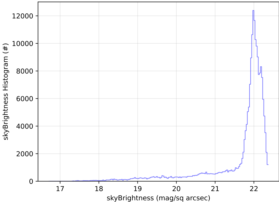
too_elab_r256_d2_griz_v3.4_10yrs All sky g band: skyBrightness Histogram
