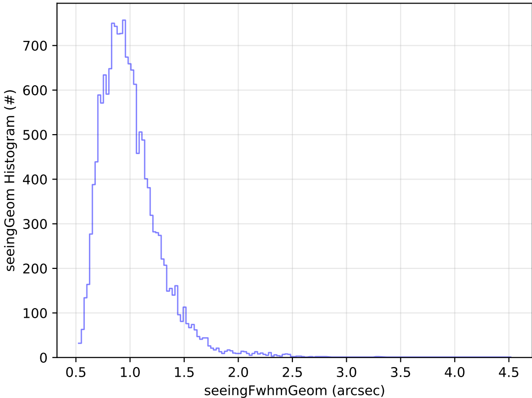
too_elab_r256_d2_griz_v3.4_10yrs Yr 1 u band: seeingGeom Histogram
