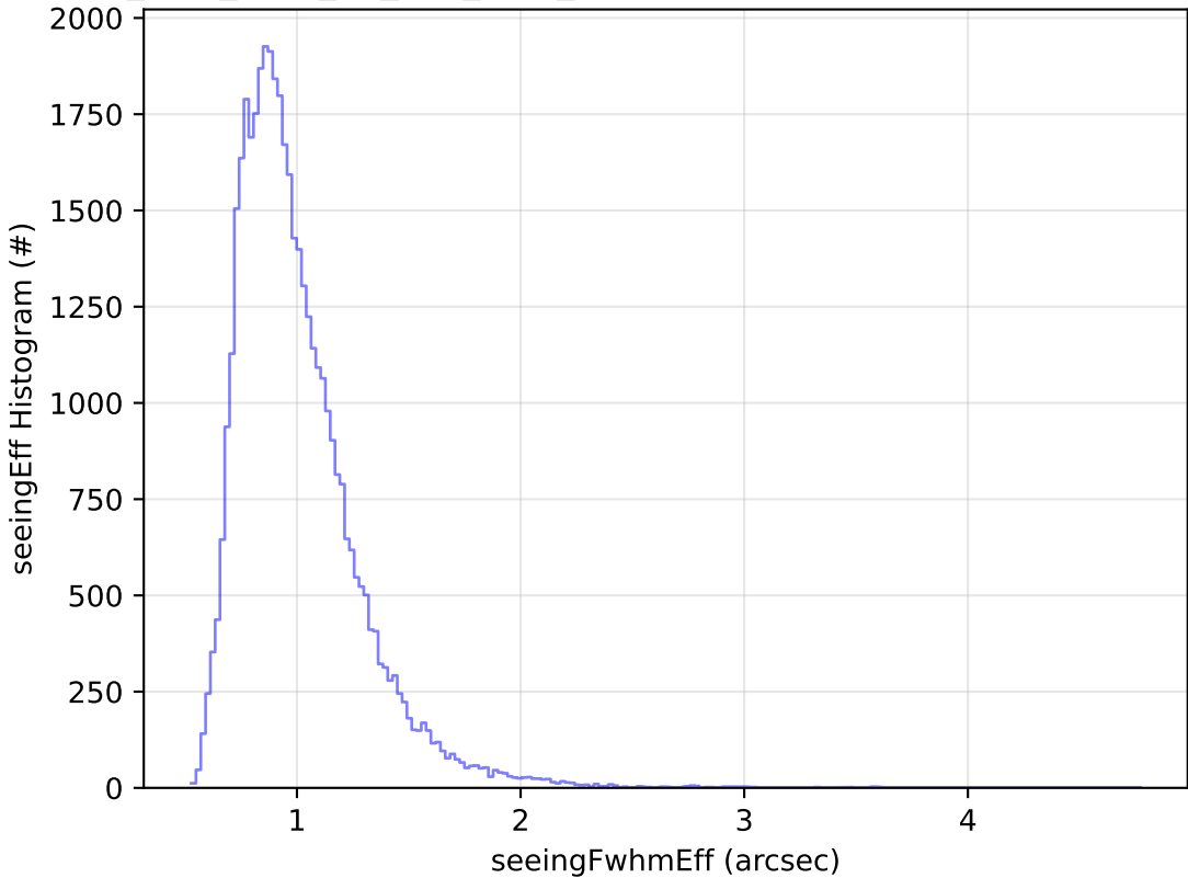
too_elab_r256_d2_griz_v3.4_10yrs Yr 1 z band: seeingEff Histogram
