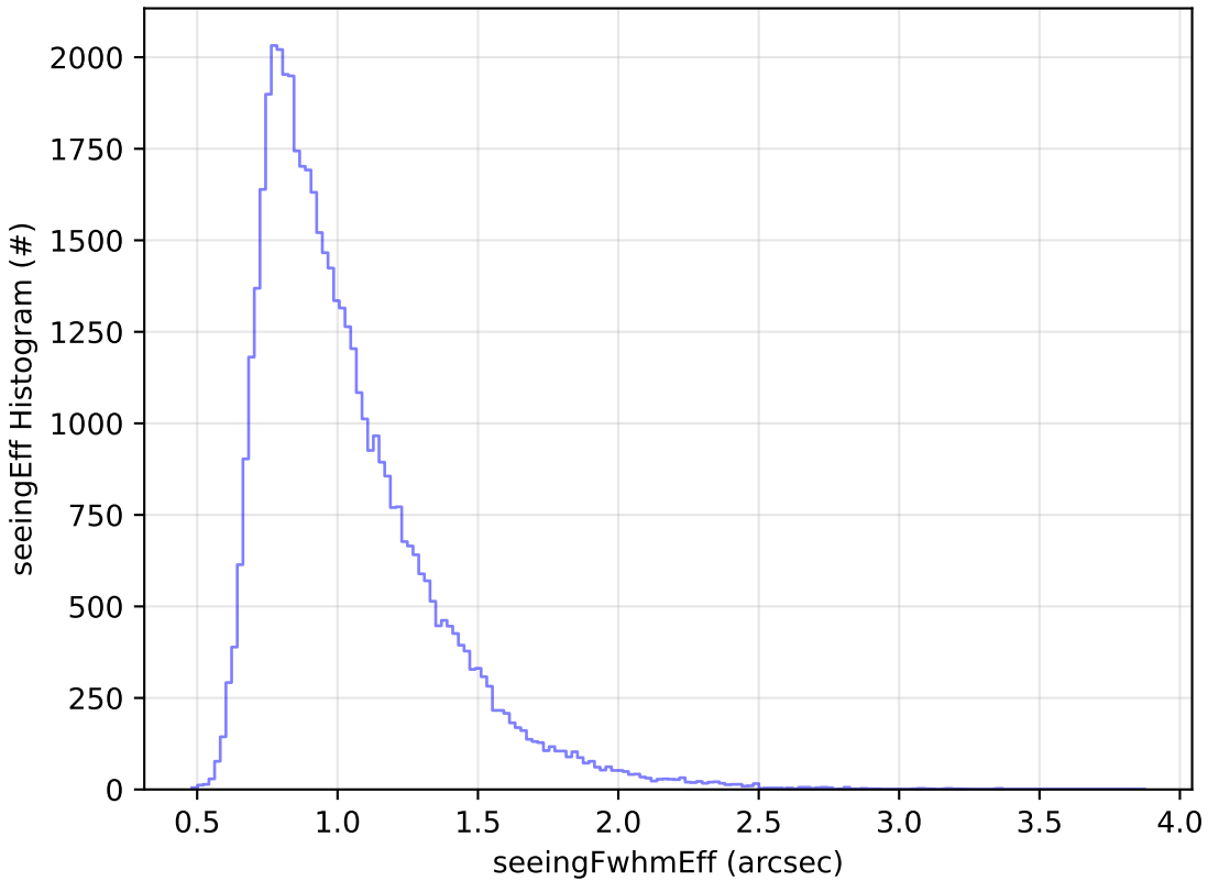
too_elab_r256_d2_griz_v3.4_10yrs Yr 1 r band: seeingEff Histogram
