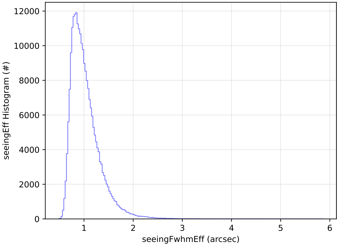
too_elab_r256_d2_griz_v3.4_10yrs Yr 1 all bands: seeingEff Histogram
