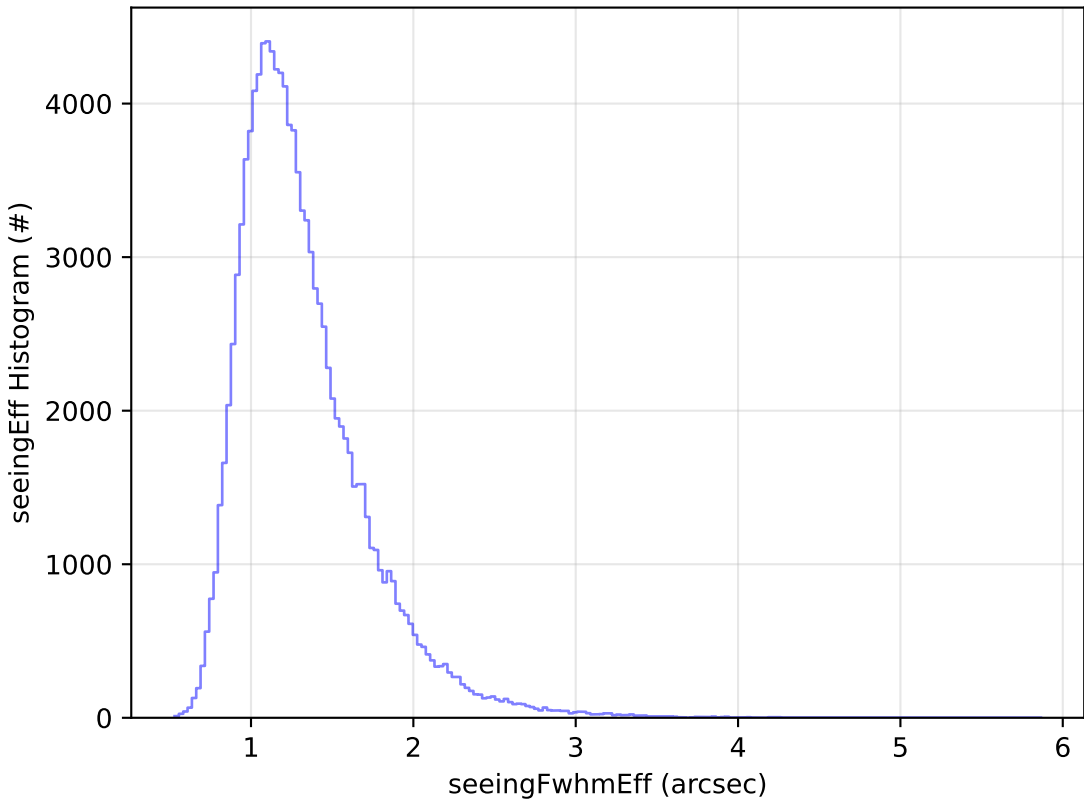
too_elab_r256_d2_griz_v3.4_10yrs WFD u band: seeingEff Histogram
