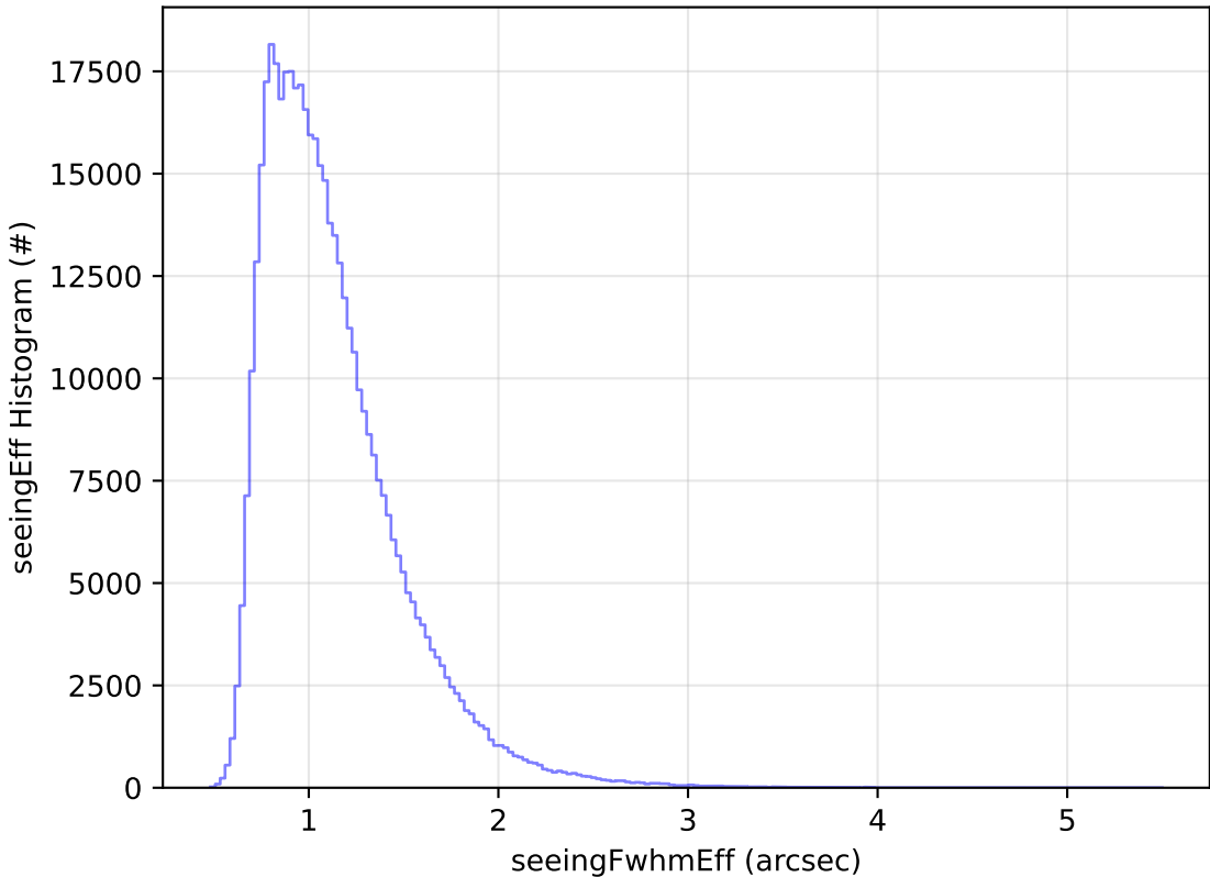
too_elab_r256_d2_griz_v3.4_10yrs WFD r band: seeingEff Histogram
