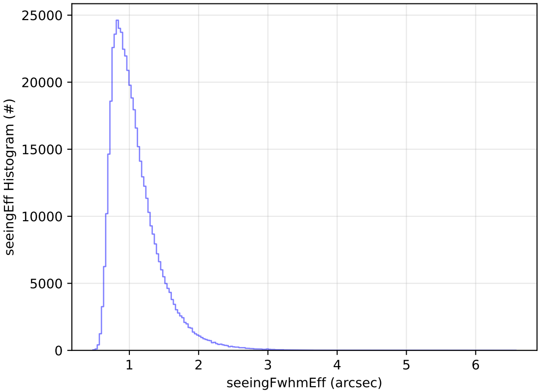
too_elab_r256_d2_griz_v3.4_10yrs WFD i band: seeingEff Histogram
