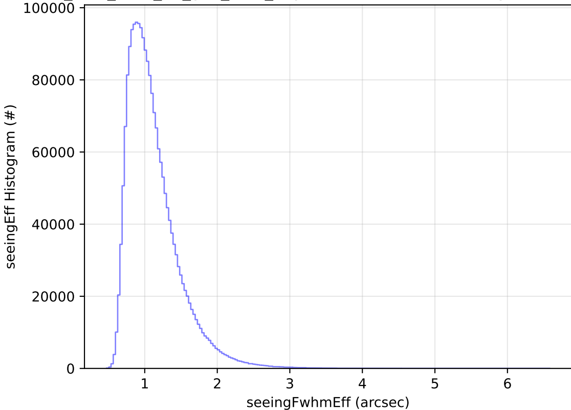
too_elab_r256_d2_griz_v3.4_10yrs WFD all bands: seeingEff Histogram
