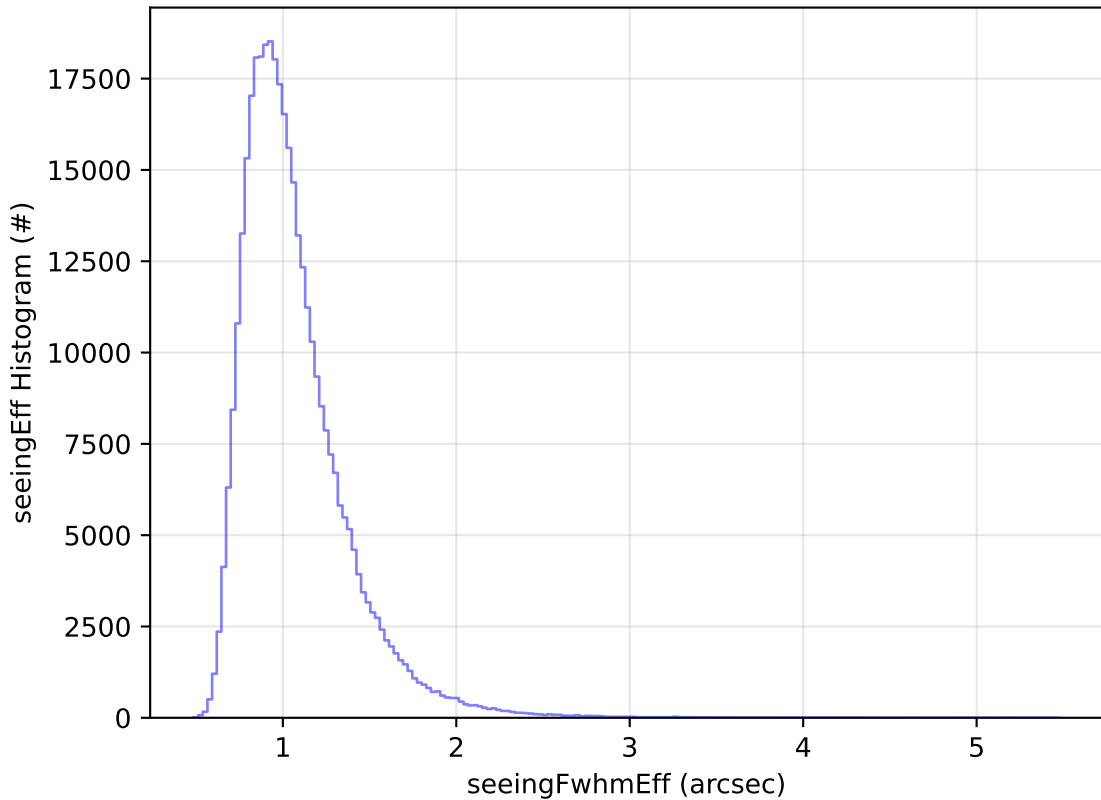
too_elab_r256_d2_griz_v3.4_10yrs All sky y band: seeingEff Histogram
