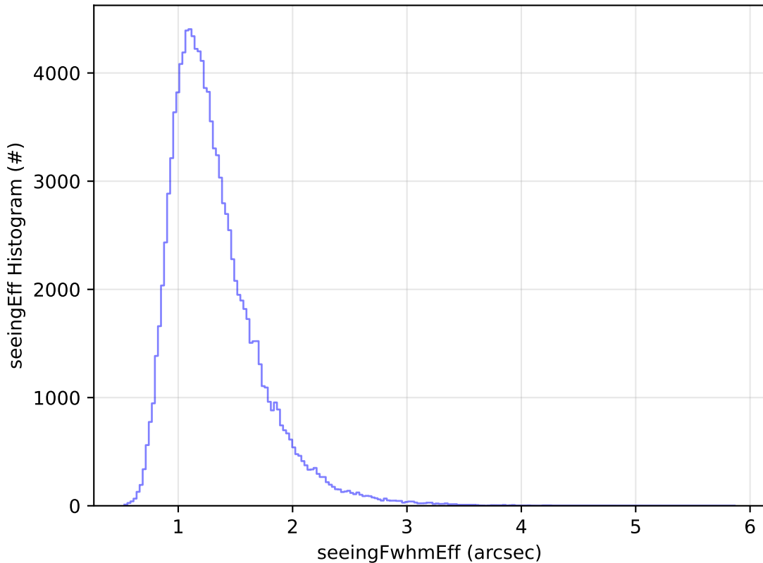
too_elab_r256_d2_griz_v3.4_10yrs All sky u band: seeingEff Histogram
